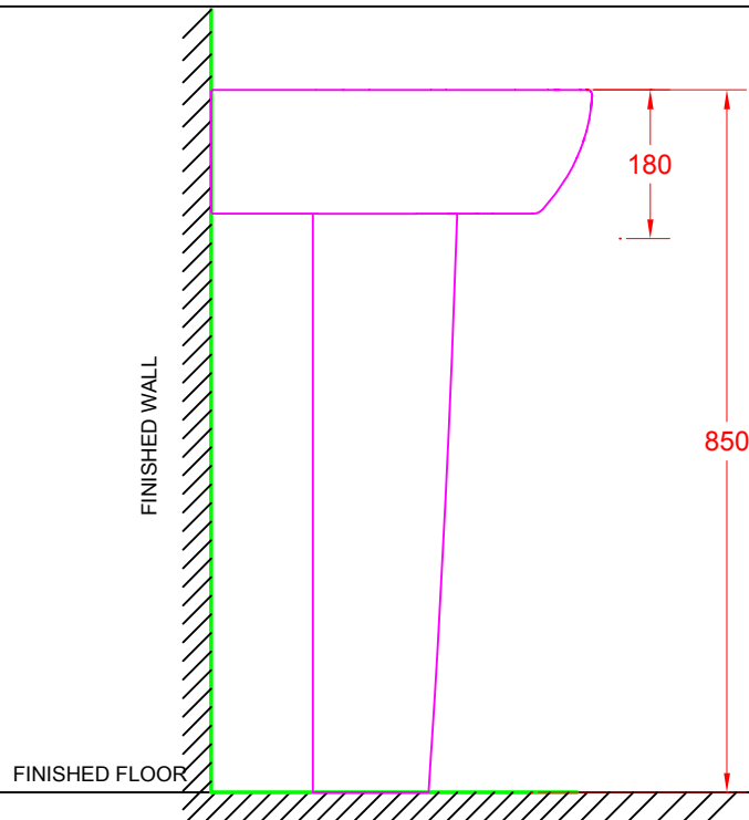
SIDE VIEW
